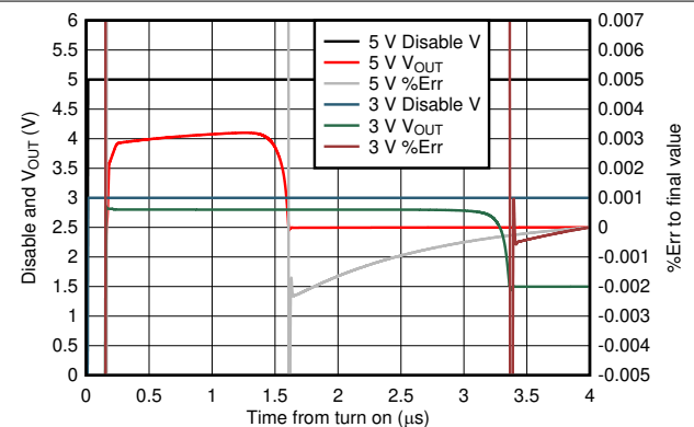
Single-supply, DC input to produce midscale output (simulation) Figure 7-54. Gain of 10-V/V Turn-On Time to Final DC Value at Midscale
