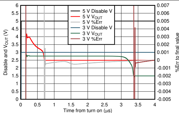
Single-supply, DC input to produce midscale output (simulation) Figure 7-53. Gain of 6-V/V Turn-On Time to Final DC Value at Midscale
