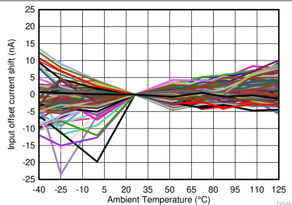
Figure 7-44. Input Offset Current Distribution
