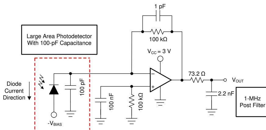
Single 3-V Supply, < 3 -mW Photodiode Amplifier With < 1.1 -pA/ \sqrt{\text{Hz}} Total Input-Referred Current Noise and 100-k \Omega Gain With Overall 1-MHz SSBW
