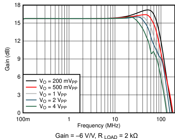
Figure 7-4. Inverting Large-Signal Bandwidth vs V_{OPP}
