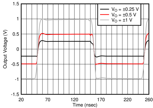
Figure 7-25. Noninverting Step Response vs V_{OPP}
