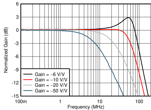
Figure 7-2. Inverting Small-Signal Frequency Response vs Gain
