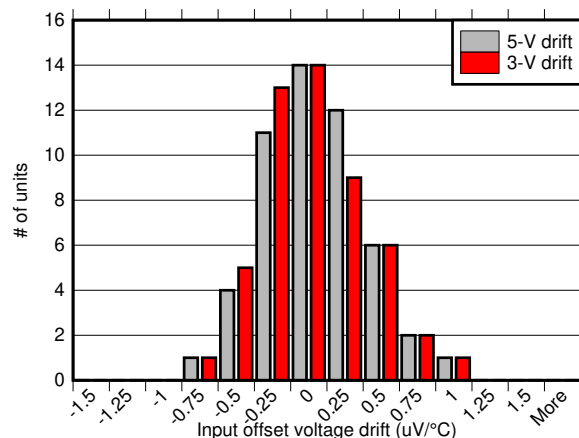
Figure 7-45. Input Offset Voltage vs Temperature
