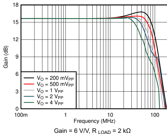
Figure 7-3. Noninverting Large-Signal Bandwidth vs V_{OPP}
