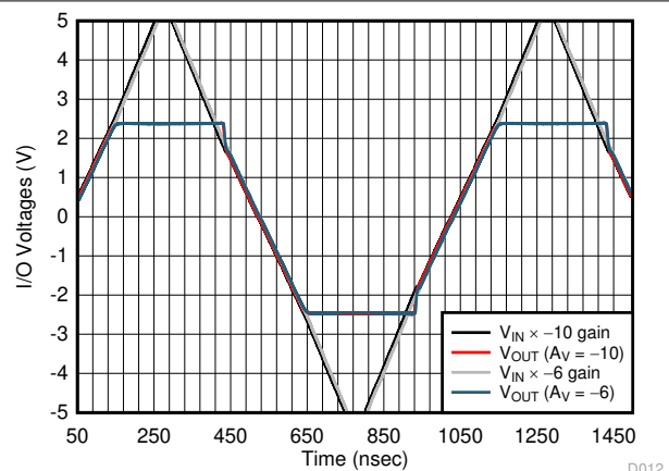
Figure 7-10. Simulated Inverting Settling Time
