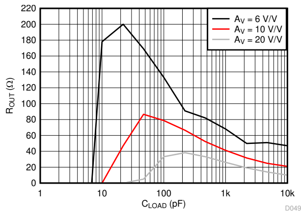
See Figure 8-6 and Table 9-1 small signal, targeting 30° phase margin Figure 7-49. Output Resistor vs C_{LOAD}
