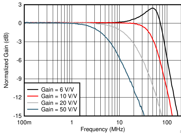
Figure 7-1. Noninverting Small-Signal Frequency Response vs Gain
