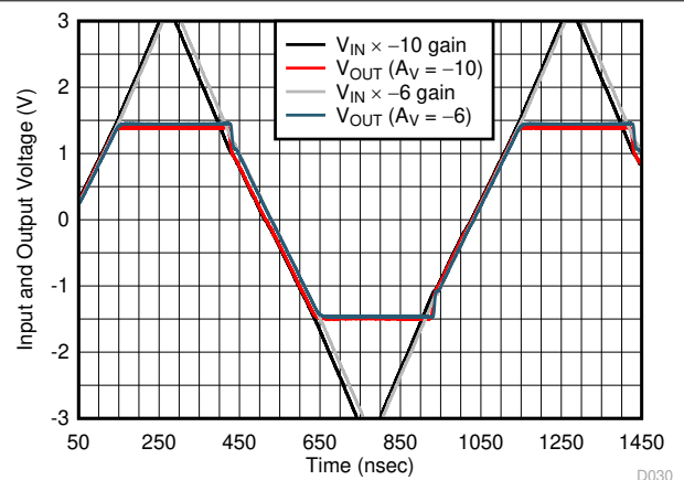
Figure 7-28. Inverting Settling Time
