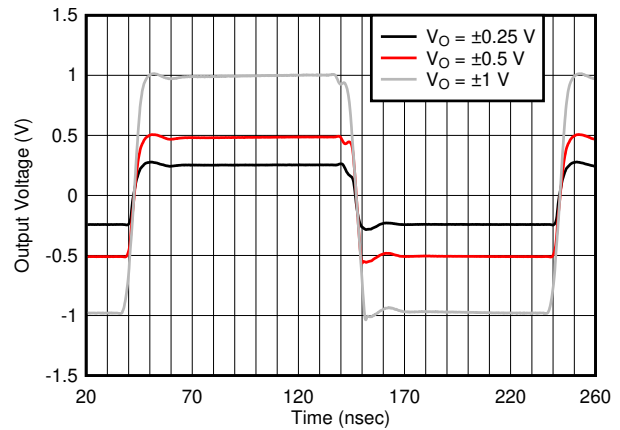
Figure 7-26. Inverting Step Response vs V_{OPP}
