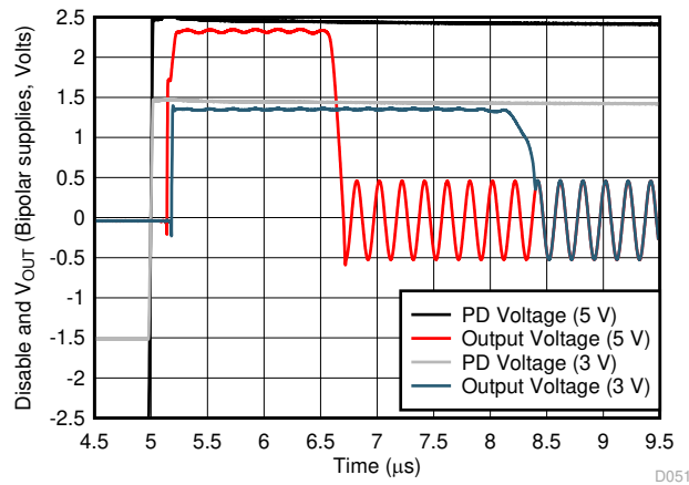
Figure 7-51. Turn-On Time to Sinusoidal Input
