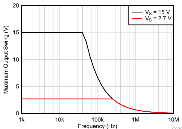
Figure 6-45. Maximum Output Voltage vs Frequency
