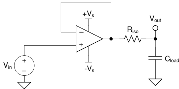
Figure 7-7. Extending Capacitive Load Drive With the OPA990
