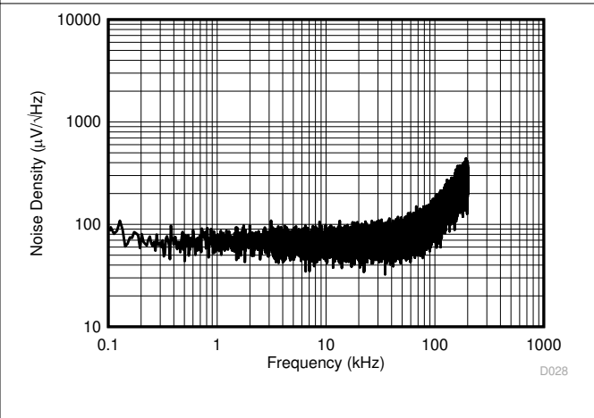
图 7-26. Input-Referred Noise Density vs Frequency
