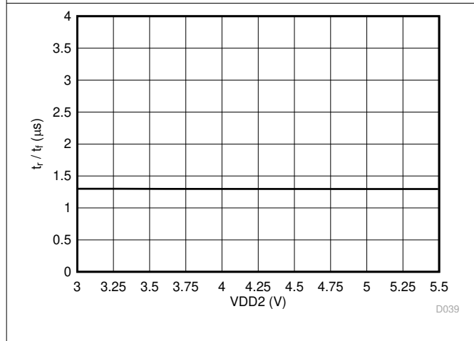
图 7-37. Output Rise and Fall Time vs Low-Side Supply
