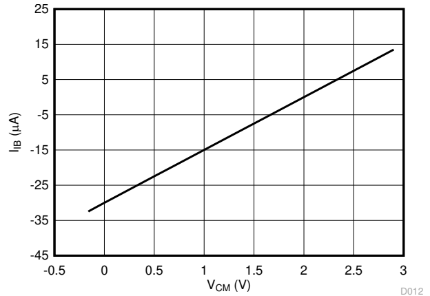
图 7-12. Input Bias Current vs Common-Mode Input Voltage
