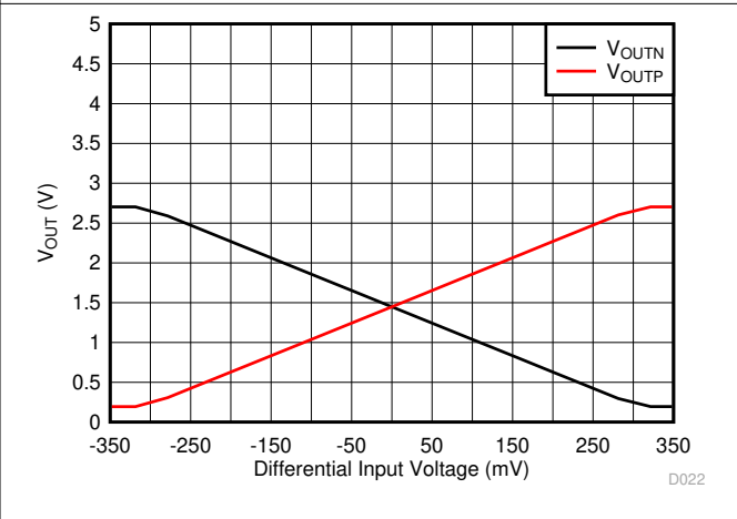
图 7-20. Output Voltage vs Input Voltage
