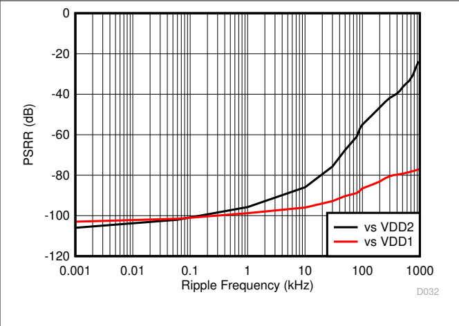
图 7-30. Power-Supply Rejection Ratio vs Ripple Frequency
