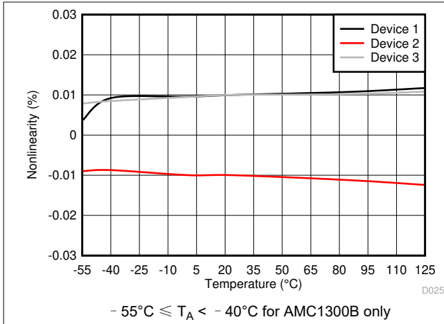
图 7-23. Nonlinearity vs Temperature
