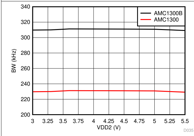
图 7-33. Output Bandwidth vs Low-Side Supply Voltage
