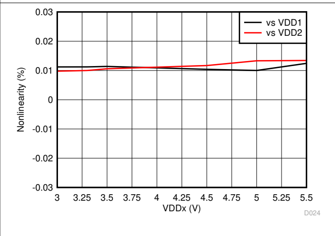
图 7-22. Nonlinearity vs Supply Voltage
