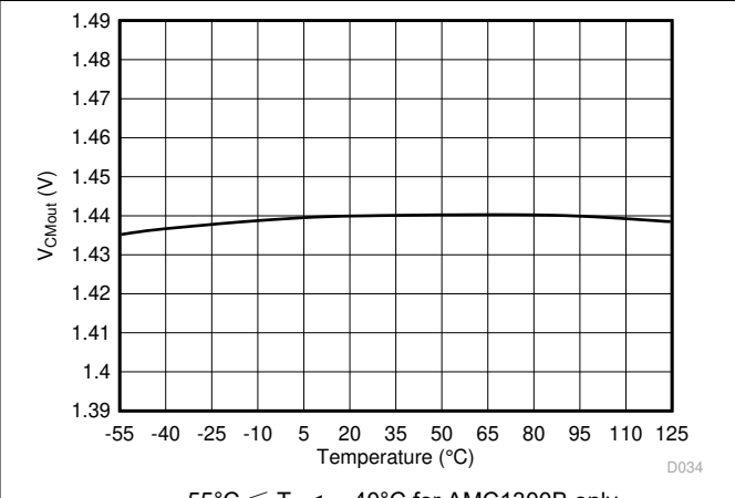
图 7-32. Output Common-Mode Voltage vs Temperature
