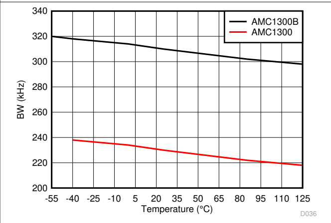
图 7-34. Output Bandwidth vs Temperature
