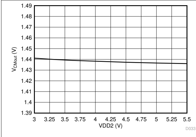
图 7-31. Output Common-Mode Voltage vs Low-Side Supply Voltage
