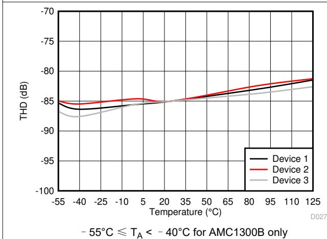
图 7-25. Total Harmonic Distortion vs Temperature
