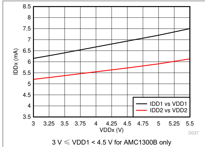
图 7-35. Supply Current vs Supply Voltage
