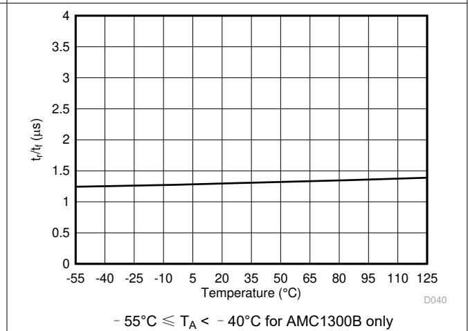
图 7-38. Output Rise and Fall Time vs Temperature
