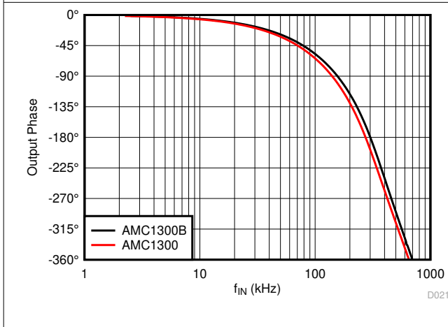
图 7-19. Output Phase vs Input Frequency
