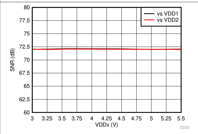
图 7-28. Signal-to-Noise Ratio vs Supply Voltage
