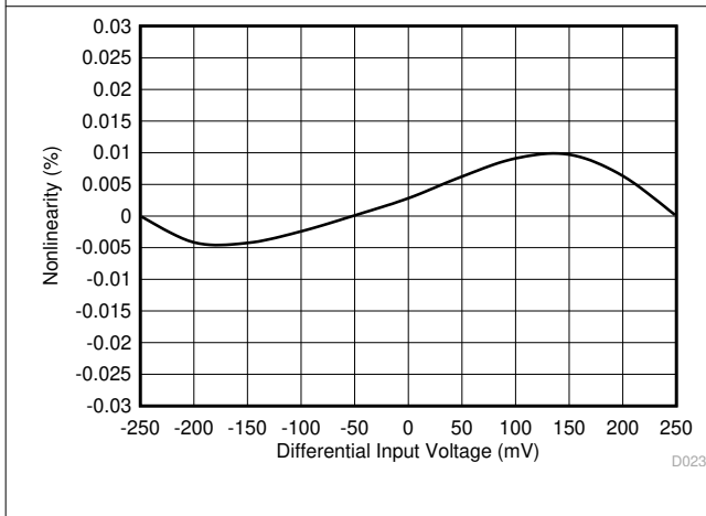
图 7-21. Nonlinearity vs Input Voltage
