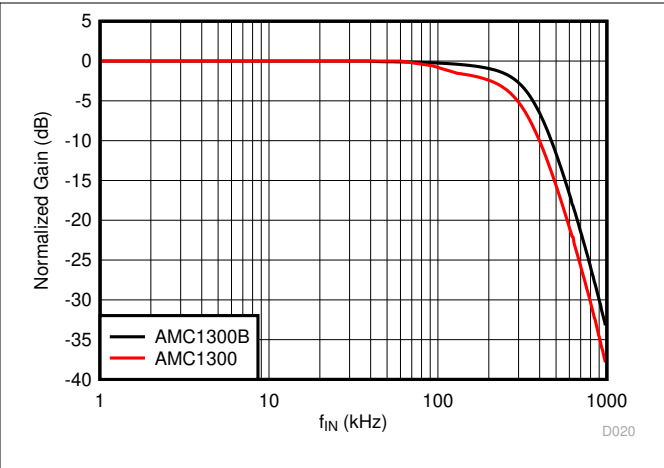
图 7-18. Normalized Gain vs Input Frequency
