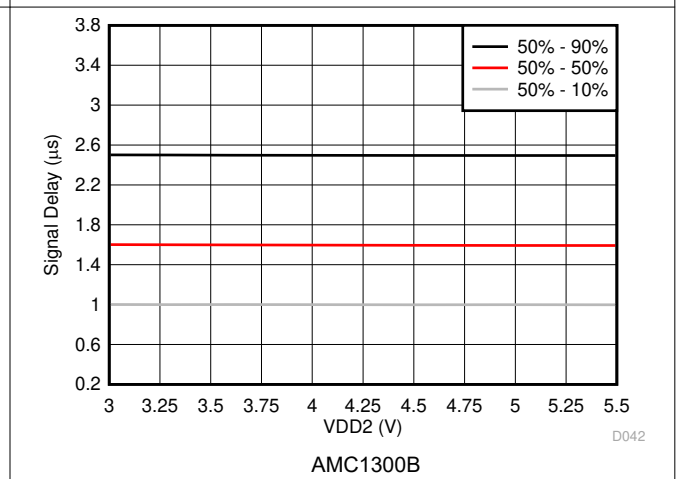
图 7-40. V IN to V OUT Signal Delay vs Low-Side Supply Voltage
