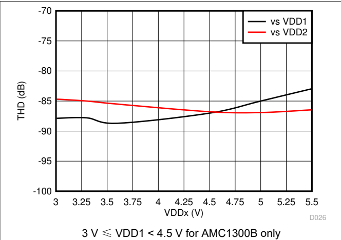
图 7-24. Total Harmonic Distortion vs Supply Voltage
