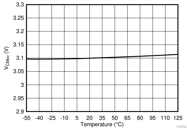
图 7-6. Common-Mode Overvoltage Detection Level vs Temperature
