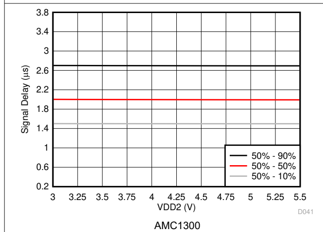
图 7-39. V IN to V OUT Signal Delay vs Low-Side Supply Voltage
