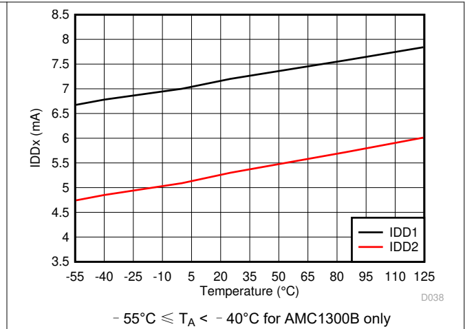
图 7-36. Supply Current vs Temperature
