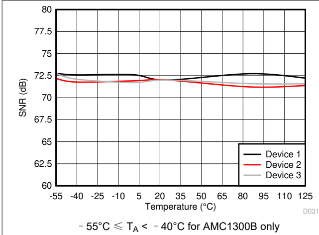
图 7-29. Signal-to-Noise Ratio vs Temperature
