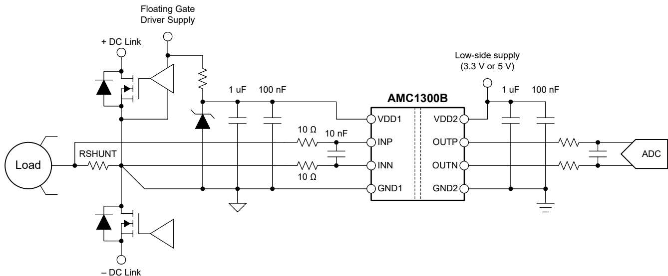
图 9-1. Using the AMC1300 for Current Sensing in a Typical Application
