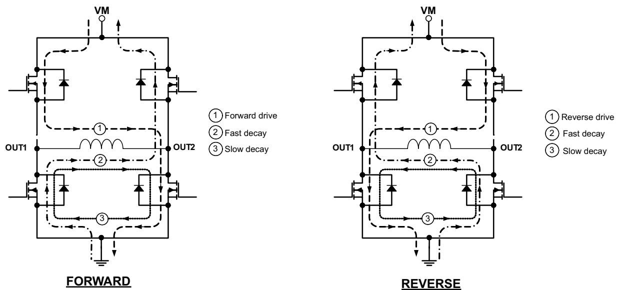
Figure 3. Current Paths
