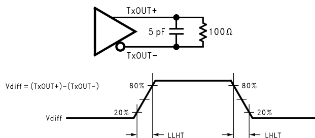
Figure 4. DS90CR217 (Transmitter) LVDS Output Load and Transition Times
