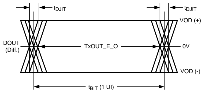
Figure 10. Output Jitter
