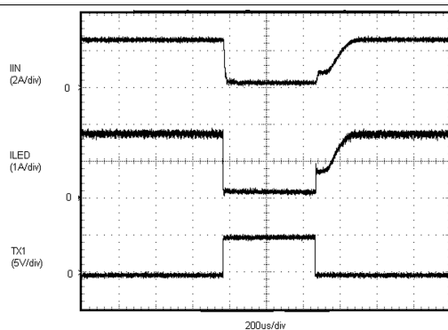
Figure 21. AET-Mode Operation
