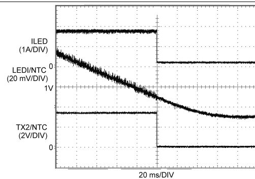
Figure 20. NTC-Mode Operation
