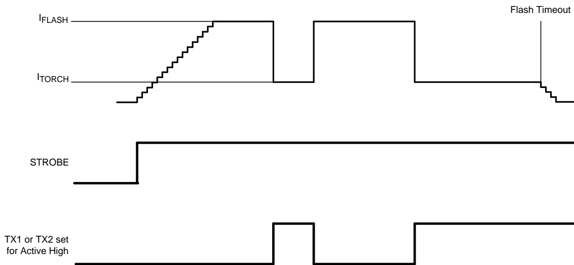
Figure 25. TX1 or TX2 Interrupt Event
