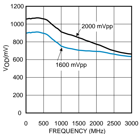
Figure 7. LVPECL with 120- \Omega Emitter Resistors V_{OD} vs Frequency
