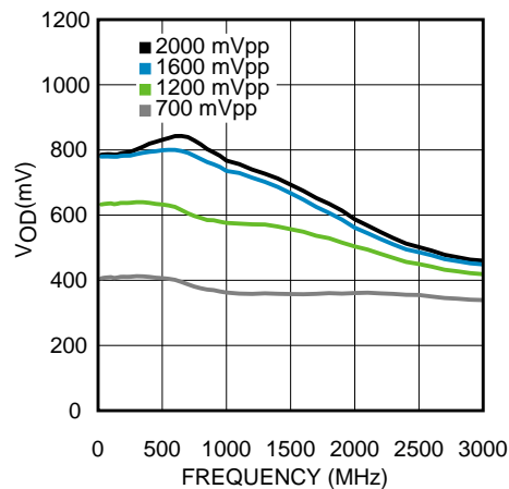
Figure 6. LVPECL with 240- \Omega Emitter Resistors V_{OD} vs Frequency
