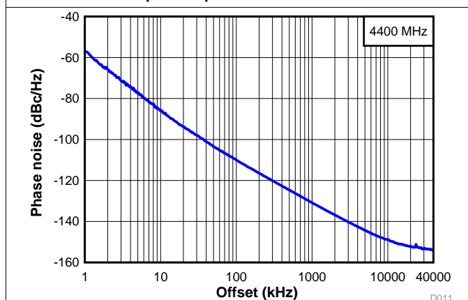
图 5. Open-Loop VCO Phase Noise at 4.4 GHz
