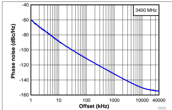
图 3. Open-Loop VCO Phase Noise at 3.4 GHz
