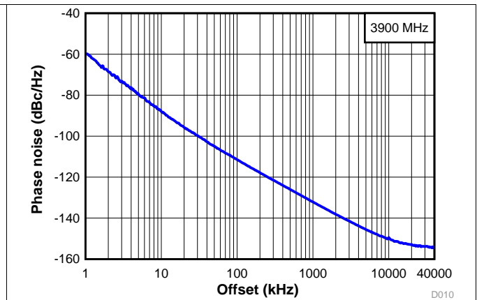
图 4. Open-Loop VCO Phase Noise at 3.9 GHz
