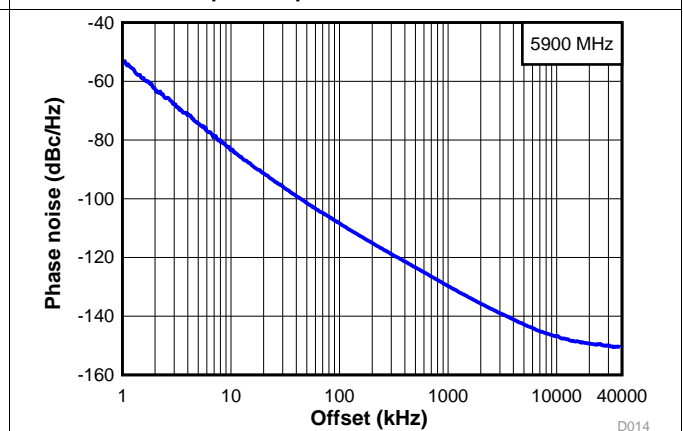
图 8. Open-Loop VCO Phase Noise at 5.9 GHz
