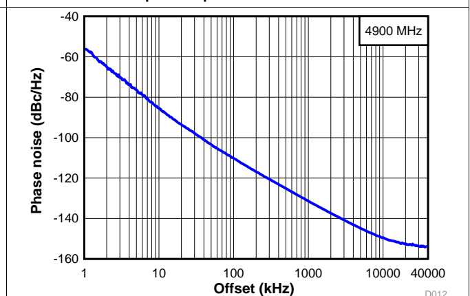
图 6. Open-Loop VCO Phase Noise at 4.9 GHz
