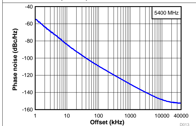
图 7. Open-Loop VCO Phase Noise at 5.4 GHz
