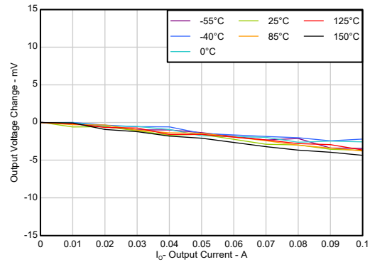
图 5-42. Load Regulation vs Load Current (New Chip)
