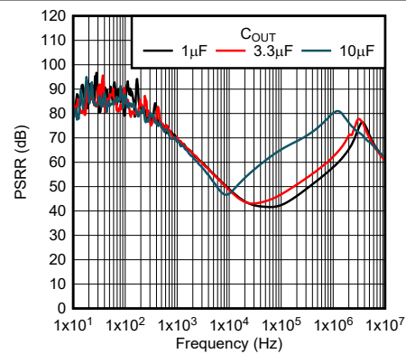
图 5-58. Ripple Rejection vs Frequency (New Chip)
