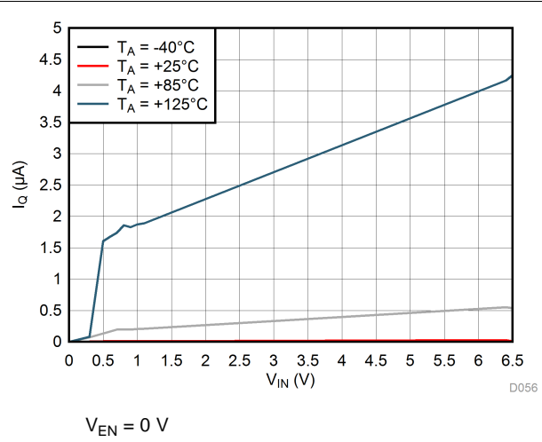
Figure 16. LP5912-3.3 I_{Q(SD)} vs V_{IN}
