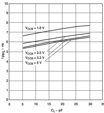
图 6-3. Typical Propagation Delay of High-to-Low (B to A) vs Load Capacitance T_A = 25^\circ\text{C} , V_{CCA} = 1.8\text{ V}
