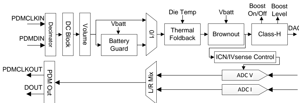
图 56. Mode 5 Processing Block Diagram
