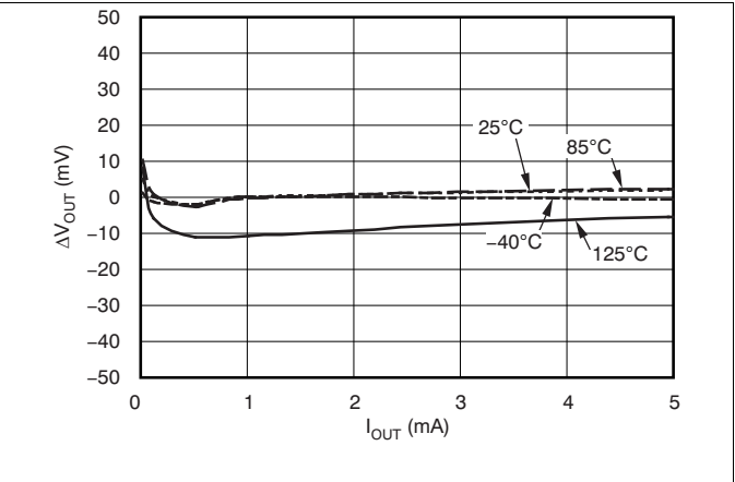
Figure 2. Load Regulation Under Light Loads
