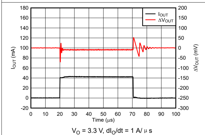
图 8-8. Load Transient Behavior for New Chip
