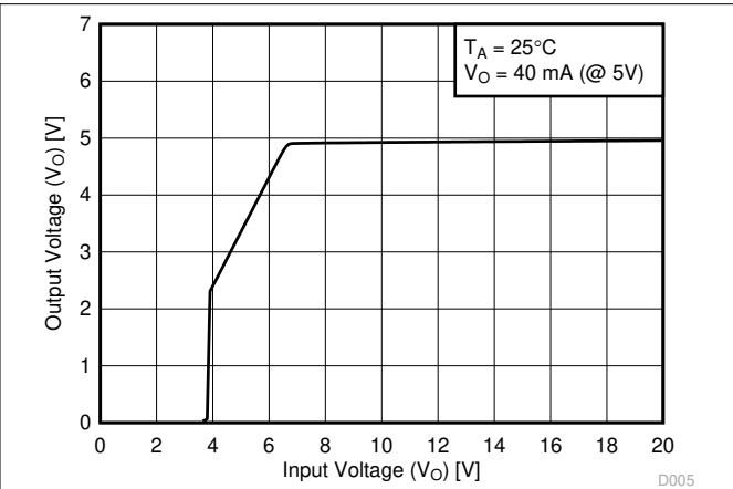
图 8-5. Output Voltage vs Input Voltage for New Chip
