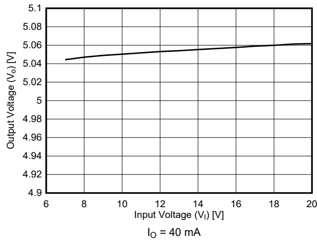
图 6-7. Line Regulation at I_O = 40\text{ mA} for New Chip at T_J = 25\text{ }^\circ\text{C}
