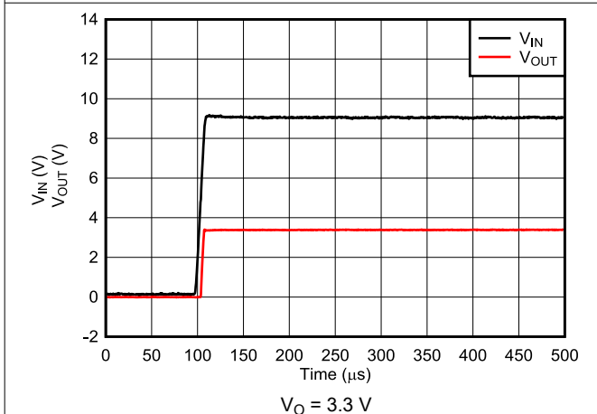
图 8-6. Start-Up With Fast V_I Ramp for New Chip
