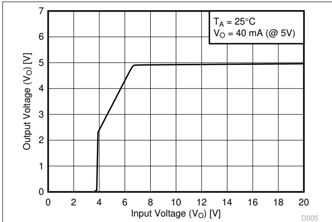
图 8-4. Output Voltage vs Input Voltage for Legacy Chip
