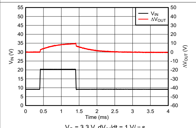
图 8-9. Line Transient Behavior for New Chip
