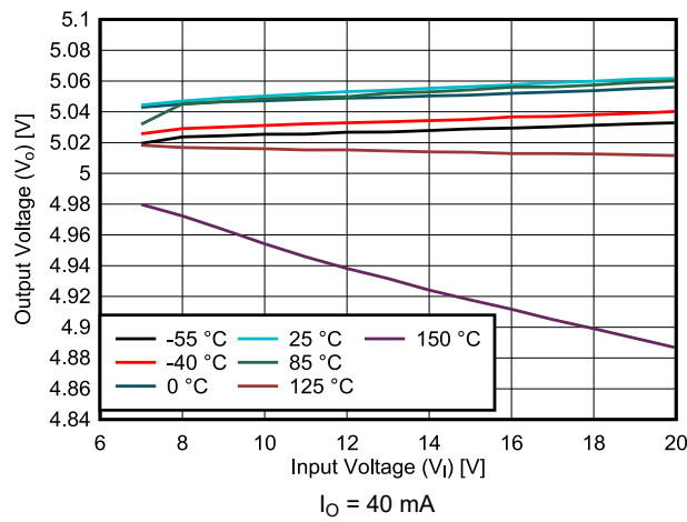
图 6-9. Line Regulation at I_O = 40\text{ mA} for New Chip
