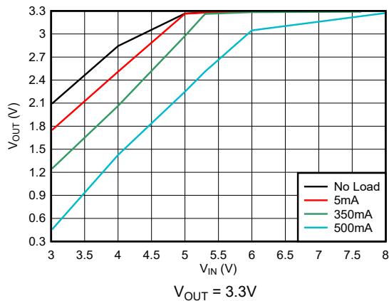
图 7-6. V_{IN} vs V_{OUT} at T_J = 25^\circ\text{C} (New Chip)
