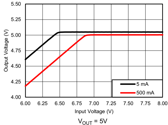
图 7-4. V_{IN} vs V_{OUT} at T_J = 25^\circ\text{C} (Legacy Chip)
