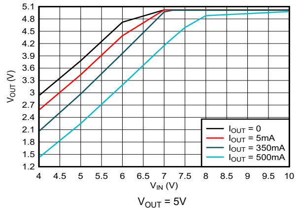
图 7-5. V_{IN} vs V_{OUT} at T_J = 25^\circ\text{C} (New Chip)
