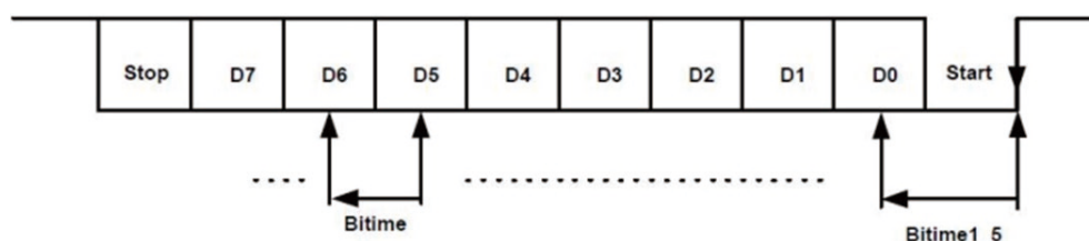
Figure 2. UART8N1 Character
