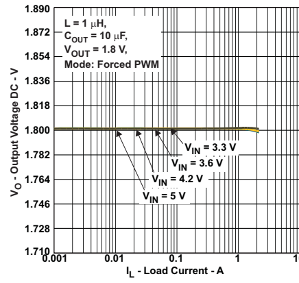
Figure 14. Forced PWM Mode
