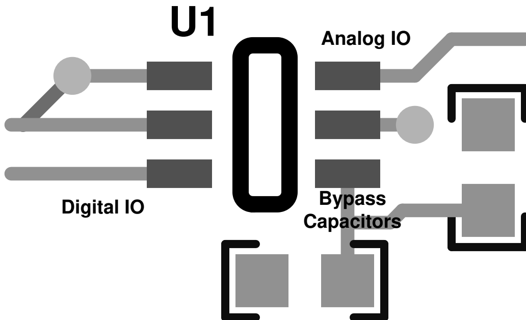
Figure 9-10. Recommended Layout
