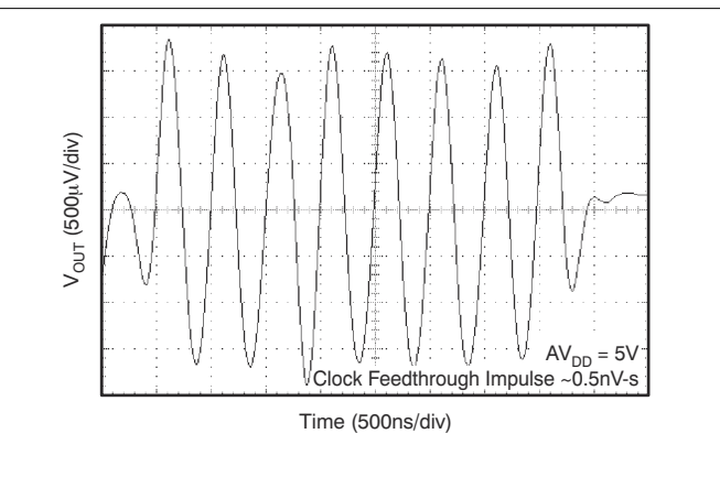
Figure 7-25. Clock Feedthrough, 5-V, 2-MHz, Midscale
