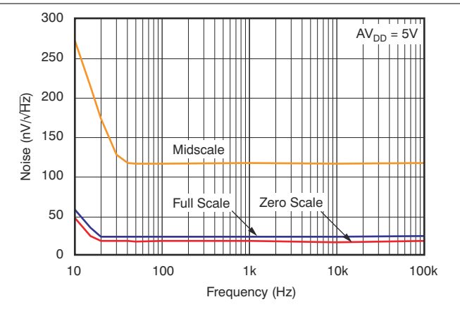
Figure 7-23. DAC Output Noise Density vs Frequency
