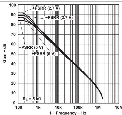
Figure 17. PSRR vs Frequency
