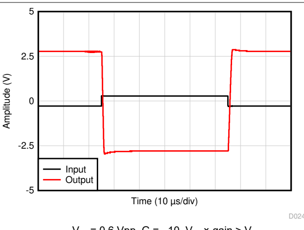
Figure 7-62. Overload Recovery
