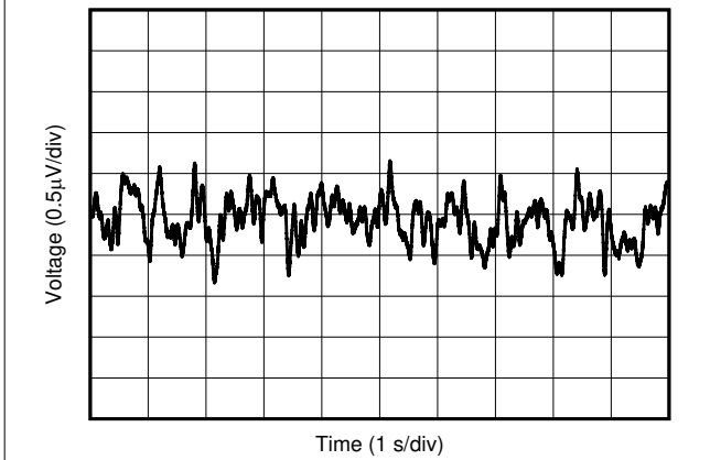
Figure 7-15. 0.1-Hz to 10-Hz Flicker Noise
