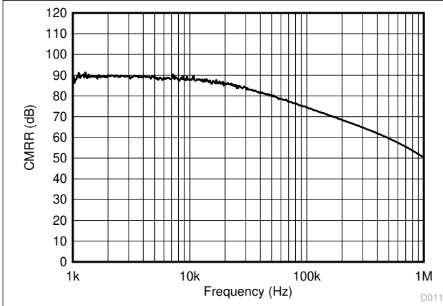
Figure 7-13. CMRR vs Frequency (Referred to Input)
