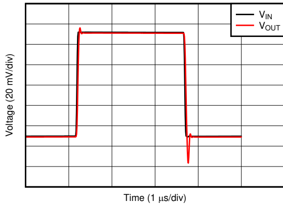
D030 V_S = 1.8\text{ V} V_{ICM} = 0.9\text{ V} V_{OCM} = 0.9\text{ V} C_L = 30\text{ pF} Gain = 1 V_{IN} = 100\text{ mVpp} Figure 7-31. Small-Signal Step Response
