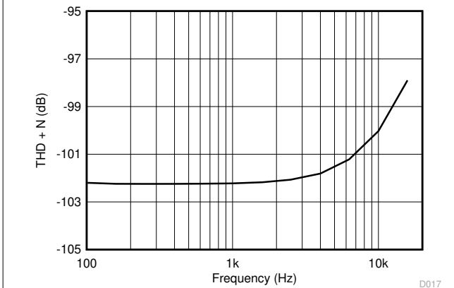
Figure 7-17. THD + N vs Frequency V_S = 5.5\text{ V} V_{ICM} = 2.5\text{ V} R_L = 2\text{ k}\Omega Gain = 1 BW = 80\text{ kHz} V_{OUT} = 0.5\text{ V}_{rms}
