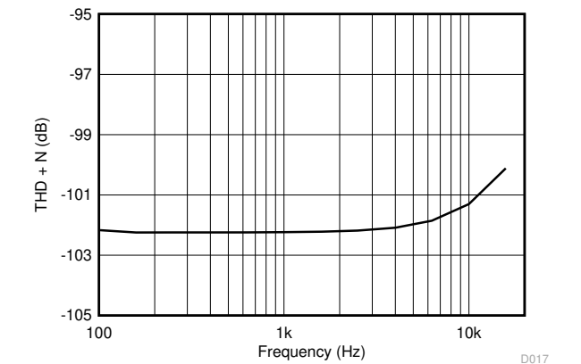
Figure 7-18. THD + N vs Frequency V_S = 5.5\text{ V} V_{ICM} = 2.5\text{ V} R_L = 10\text{ k}\Omega Gain = 1 BW = 80\text{ kHz} V_{OUT} = 0.5\text{ V}_{rms}
