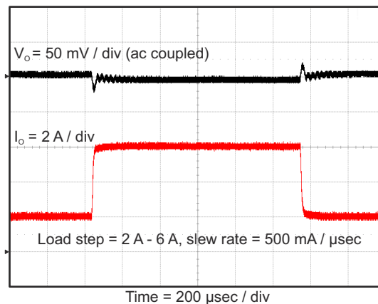
Figure 8-18. Transient Response
