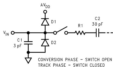
Figure 25. Equivalent Input Circuit
