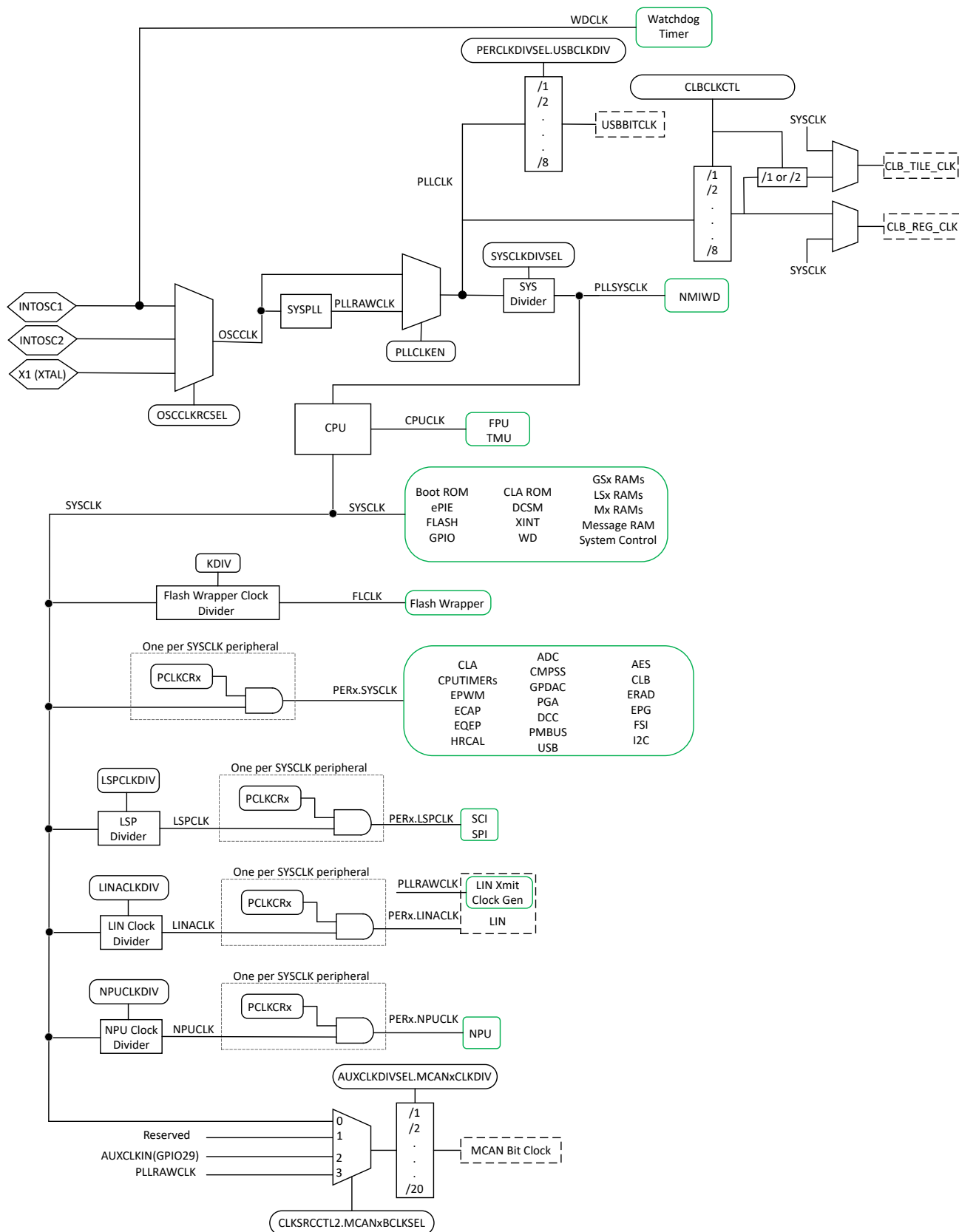
Figure 6-9. Clocking System
