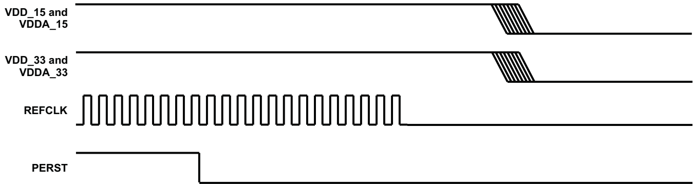
Figure 3-3. Power-Down Sequence
