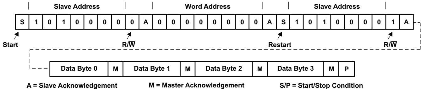
Figure 3-11. Serial-Bus Protocol Multibyte Read
