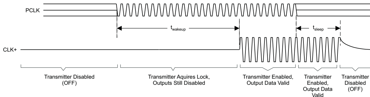
Figure 14. Standby Detection
