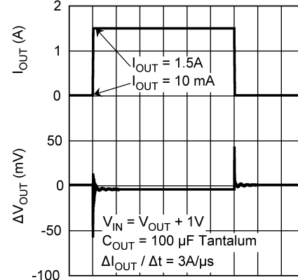
Load Transient Response, C_{OUT} = 100\ \mu\text{F Tantalum}
