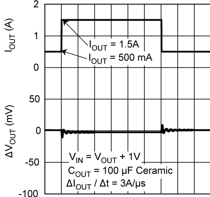
Load Transient Response, C_{OUT} = 100\ \mu\text{F Ceramic}
