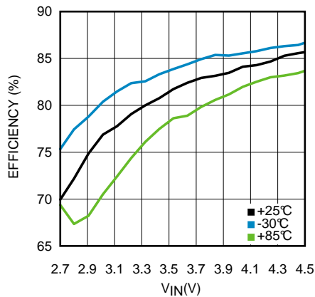
Figure 5. LED Efficiency vs Input Voltage at 930mA
