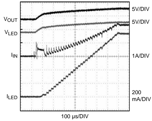
Figure 26. Flash Ramp-Up
