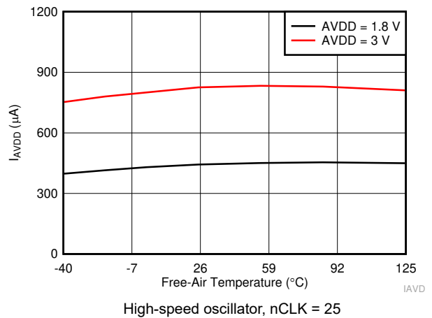
Figure 6-36. I_{AVDD} in High-Precision Mode vs Temperature High-speed oscillator, nCLK = 25
