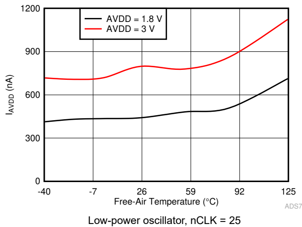
Figure 6-35. I_{AVDD} in High-Precision Mode vs Temperature Low-power oscillator, nCLK = 25
