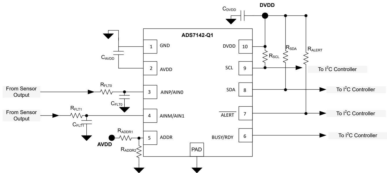
Figure 8-10. Example Schematic
