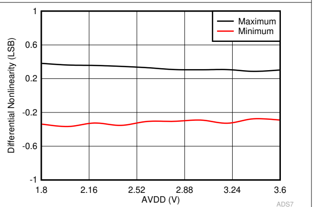
Figure 6-22. DNL in Manual Mode vs AVDD
