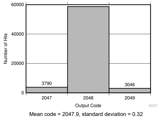
Figure 6-12. Typical DC Code Spread in Manual Mode
