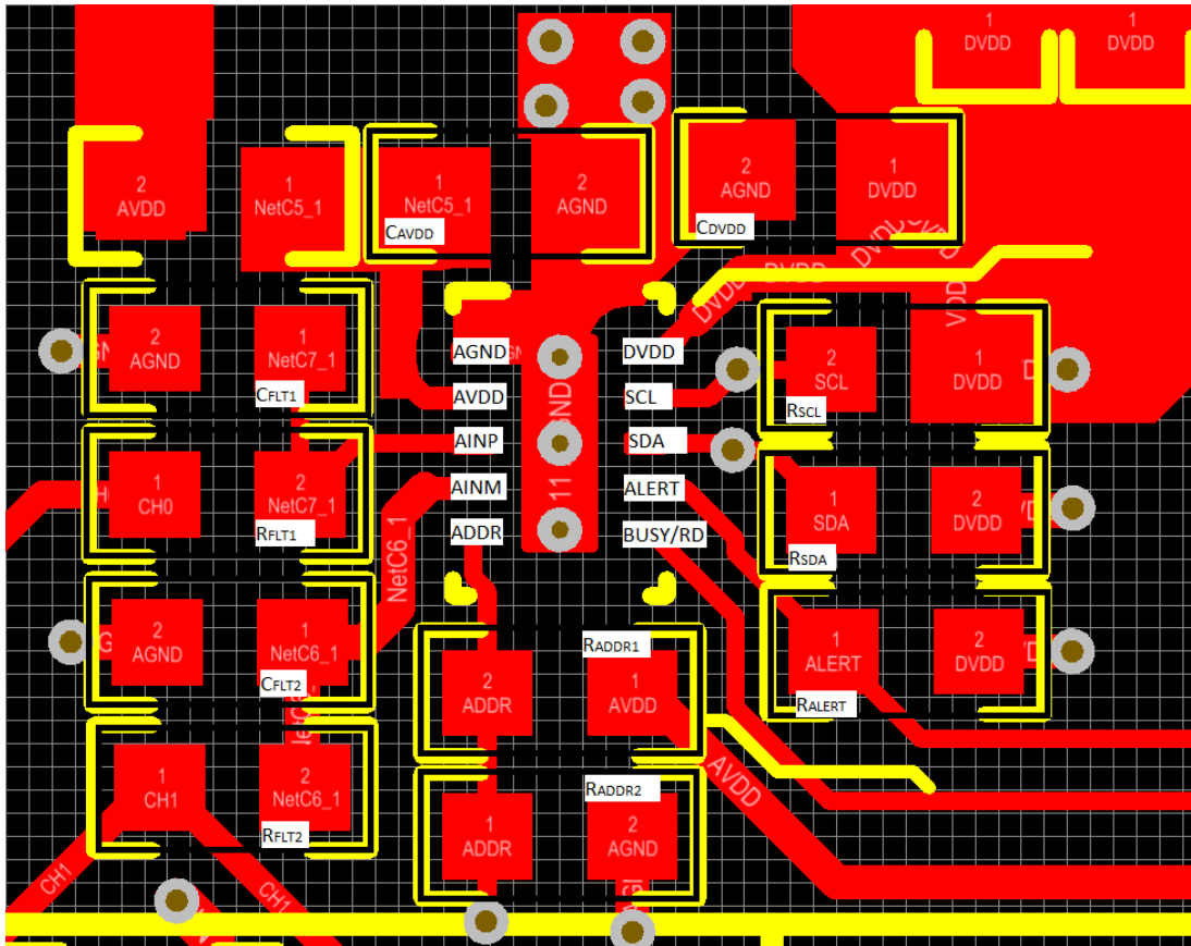
Figure 8-11. Example Layout
