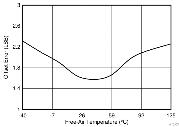
Figure 6-13. Offset Error in Manual Mode vs Temperature
