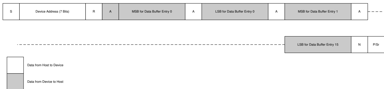
Figure 7-8. Reading Data Buffer (16 Bit Words × 16 Words)
