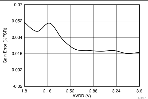
Figure 6-16. Gain Error in Manual Mode vs AVDD
