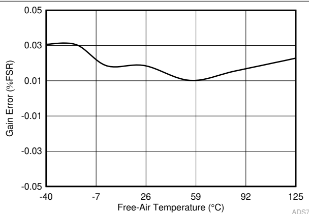
Figure 6-15. Gain Error in Manual Mode vs Free-Air Temperature
