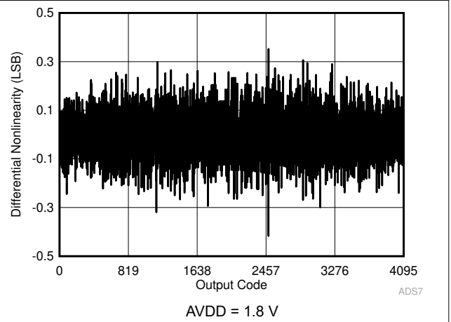
Figure 6-18. Typical DNL in Manual Mode
