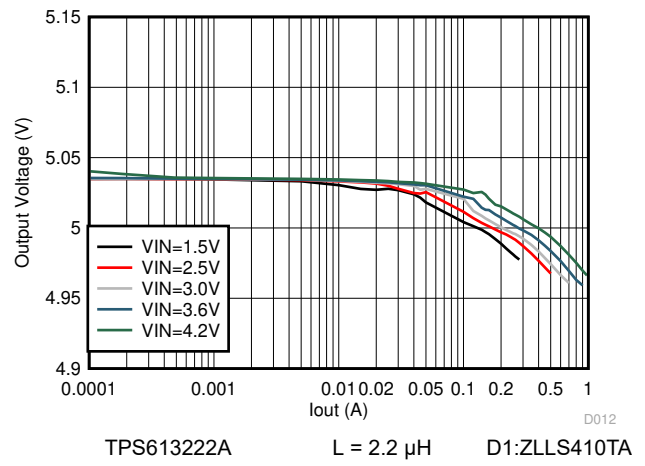
Figure 8-19. Load Regulation
