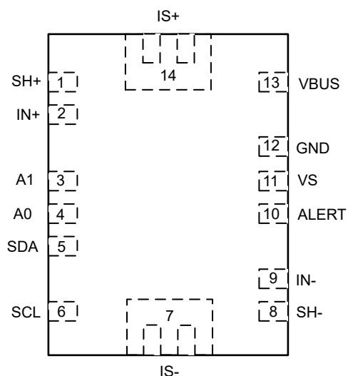
Figure 5-1. REM Package 14-Pin QFN Top View
