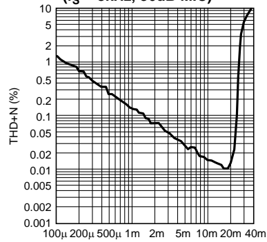
MIC INPUT VOLTAGE (Vrms)
