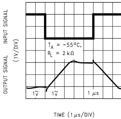
Figure 5-33. Inverting Large Signal Pulse Response
