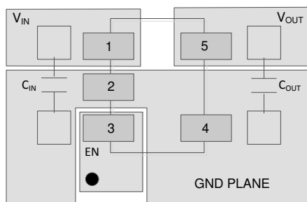
Figure 9-1. WSON Layout Example
