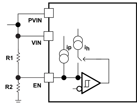
Figure 32. Adjustable VIN and PVIN Under Voltage Lock Out
