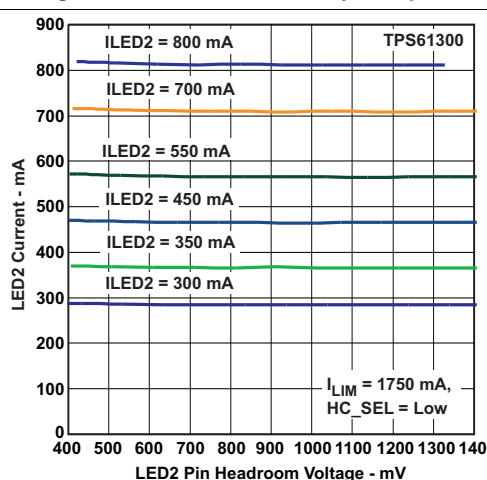
Figure 7. LED2 Current vs LED2 Pin Headroom Voltage (HC_SEL = 0)
