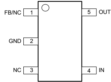
Figure 4-2. DCK Package, 5-Pin SC70 (Top View)
