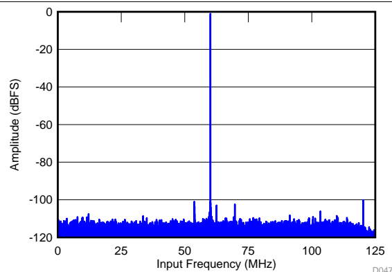
\text{SNR} = 76.4\text{ dBFS} , \text{SFDR} = 99\text{ dBc}
