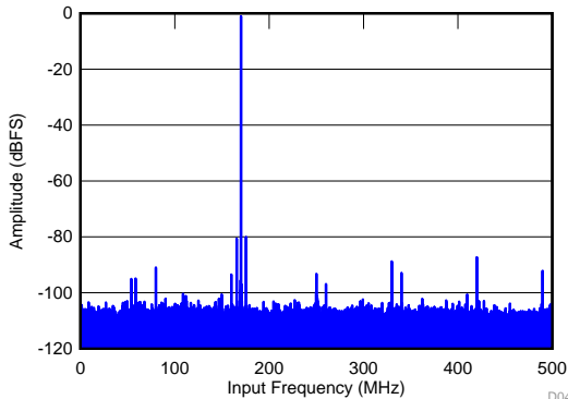
f_{\text{IN}} = 170\text{ MHz} , A_{\text{IN}} = -1\text{ dBFS} , f_{\text{CMRR}} = 5\text{ MHz} , A_{\text{CMRR}} = 50\text{ mV}_{\text{PP}} , \text{SINAD} = 69.1\text{ dBFS} , \text{SFDR} = 86\text{ dBc} , amplitude of f_{\text{IN}} \pm f_{\text{CMRR}} = -80\text{ dBFS}
