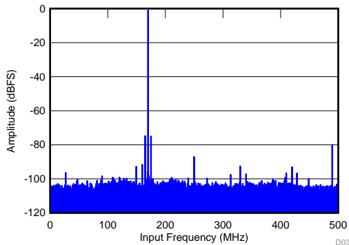
f_{\text{IN}} = 170\text{ MHz} , A_{\text{IN}} = -1\text{ dBFS} , \text{SINAD} = 67\text{ dBFS} , \text{SFDR} = 79\text{ dBc} , f_{\text{PSRR}} = 5\text{ MHz} , A_{\text{PSRR}} = 25\text{ mV}_{\text{PP}} , amplitude of f_{\text{IN}} - f_{\text{PSRR}} = -74\text{ dBFS} , amplitude of f_{\text{IN}} + f_{\text{PSRR}} = -76\text{ dBFS}
