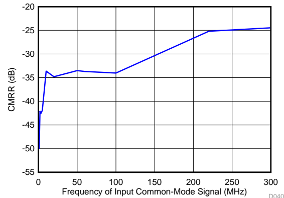
f_{\text{IN}} = 170\text{ MHz}
