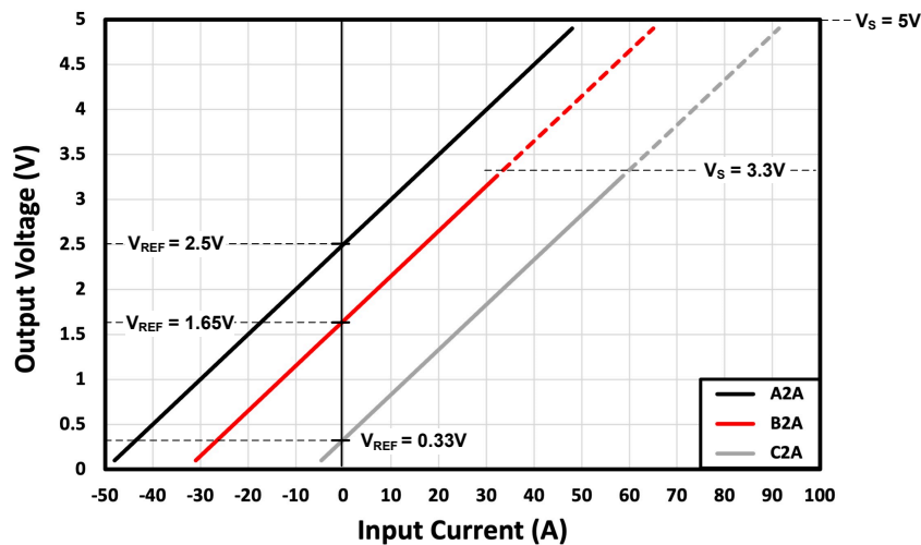
Figure 8-4. Output Voltage Relationship to Input Current for TMCS1126x2A
