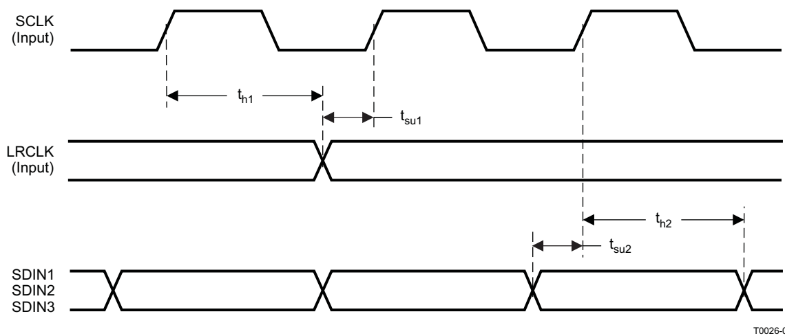
Figure 8. Slave Mode Serial Data Interface Timing
