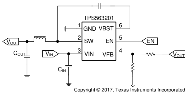
Simplified Schematic
