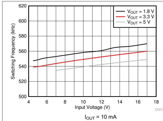
Figure 5-7. TPS563208 Switching Frequency vs Input Voltage
