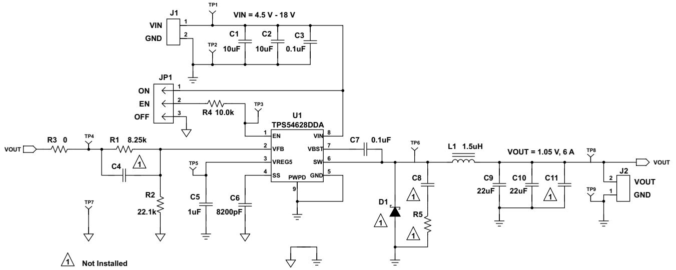
Figure 6-1. TPS54628EVM-052 Schematic Diagram
