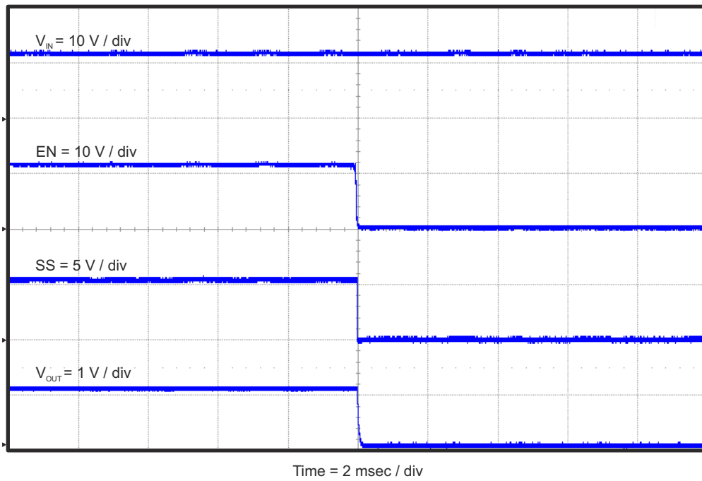
Figure 4-13. TPS54628EVM-052 Shut-Down Relative to EN with SS
