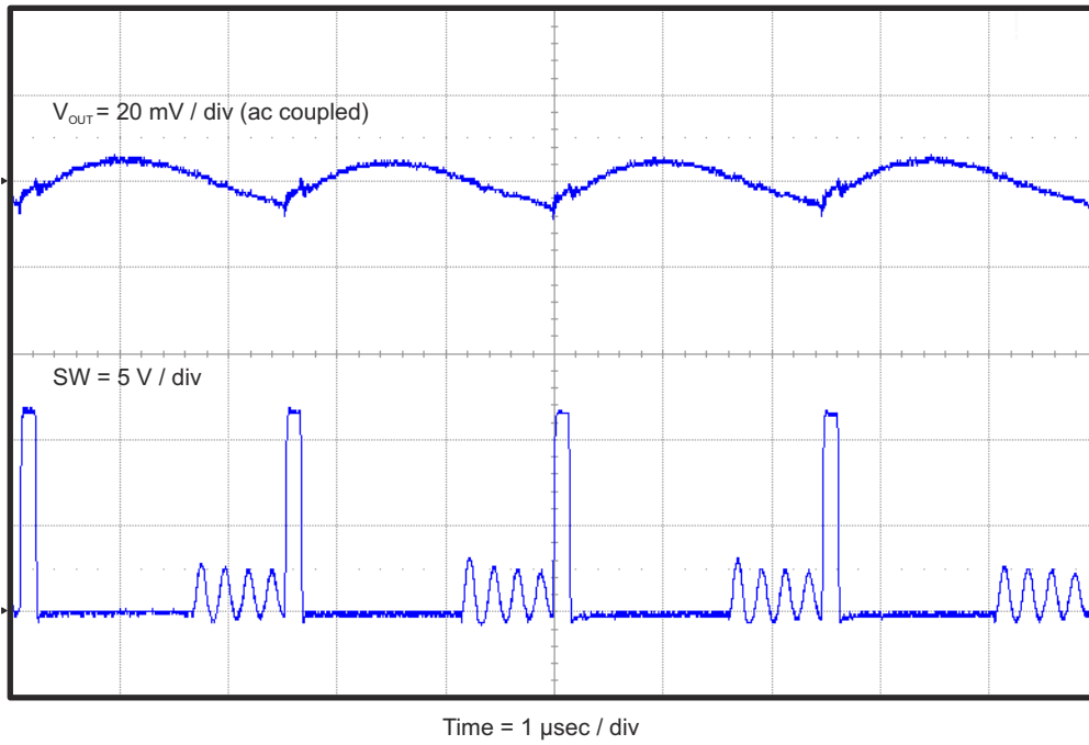
Figure 4-7. TPS54628EVM-052 Output Voltage Ripple ( I_{OUT} = 300 \text{ mA} )
