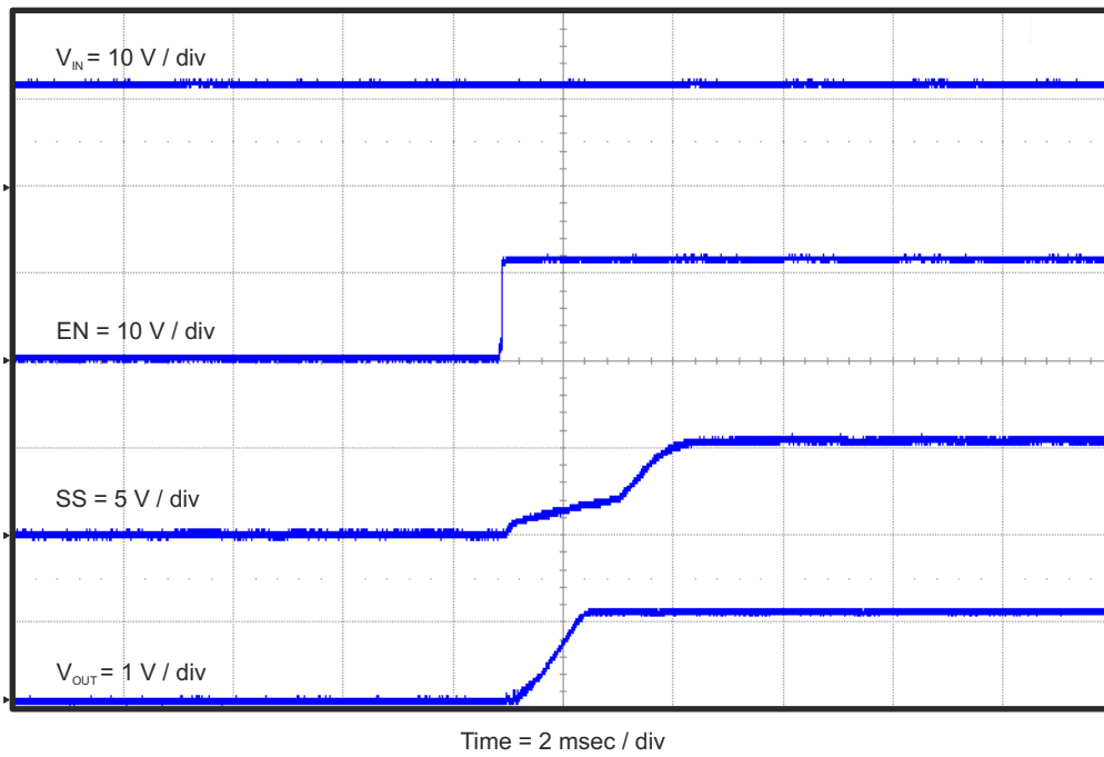
Figure 4-11. TPS54628EVM-052 Start-Up Relative to EN with SS
