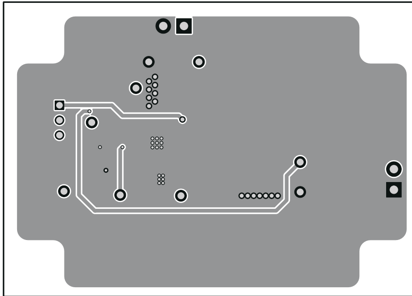
Figure 5-5. Bottom Layer
