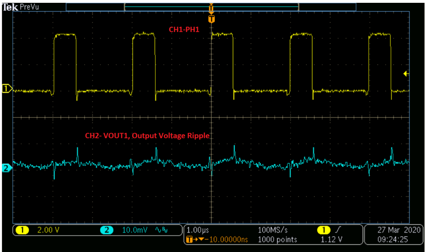
Figure 4. Output Voltage Ripple VIN = 5 V, VOUT = 1 V, IOU = 18 A
