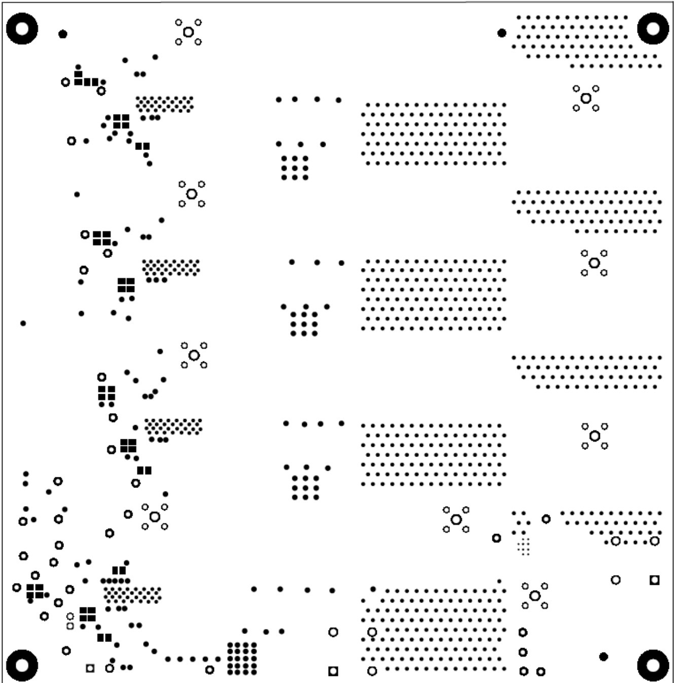
Figure 25. Bottom Solder
