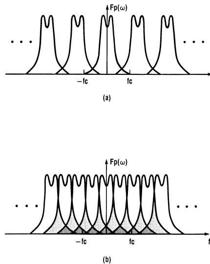
Figure 5. Spectral folding or aliasing caused by: (a) under sampling (b) exaggerated under sampling.
