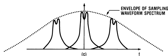
Figure 10. (c) equals the convolution of (a) with (b).
