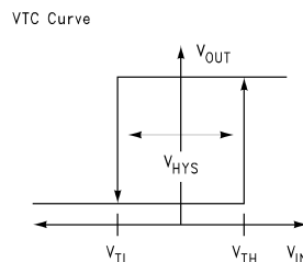
Figure 4. Hysteresis Voltage
