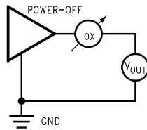
Figure 13. I_{ox} Test Circuit
