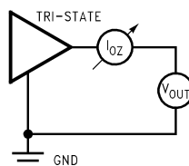
Figure 12. I_{OZ} Test Circuit
