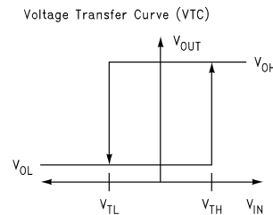
Figure 3. Threshold Voltages
