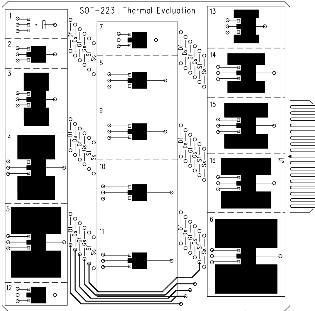
Figure 10. SOT-223 Thermal Board Top View in Actual Scale
