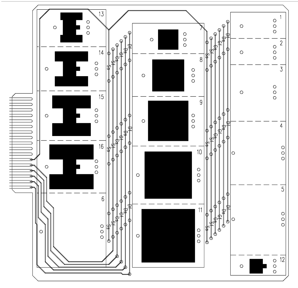
Figure 11. SOT-223 Thermal Board Bottom View in Actual Scale
