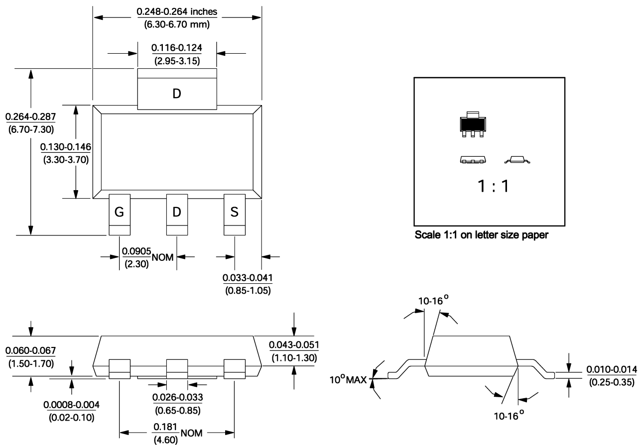
Figure 9. SOT-223
