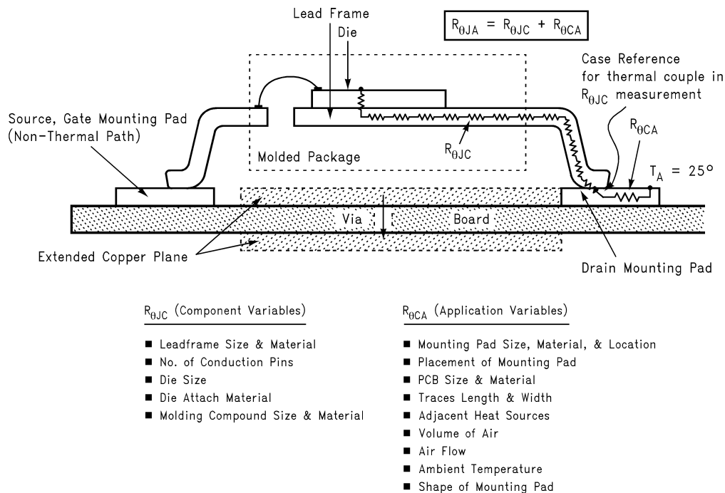
Figure 5. Cross-Sectional View of a Power MOSFET Mounted on a Printed Circuit Board
