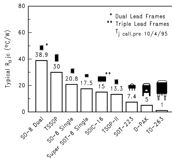
Figure 8. Junction-to-Case Thermal Resistance R_{\theta JC} of Various Surface Mount Packages
