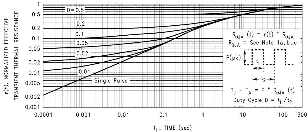
Figure 7. Normalized Transient Thermal Resistance Curves
