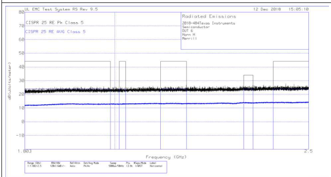
Figure 42. Radiated EMI Log Horizontal vs. CISPR25 Limits
