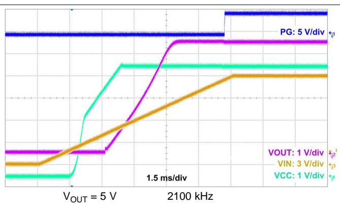
Figure 51. Start-Up Waveform
