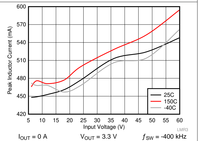
Figure 6. I_{PEAK-MIN}
