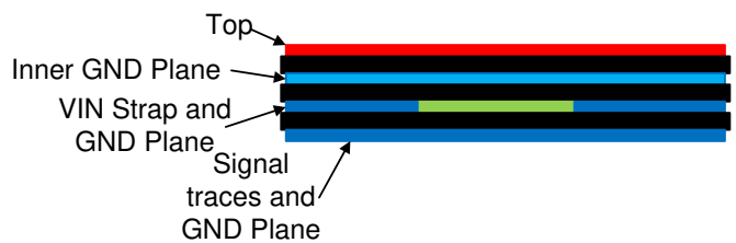
Figure 54. Example Layout
