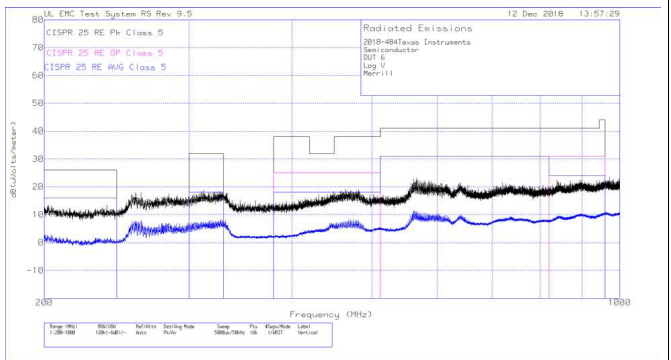
Figure 41. Radiated EMI Log Vertical vs. CISPR25 Limits
