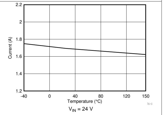
Figure 4. Low Side Current Limit
