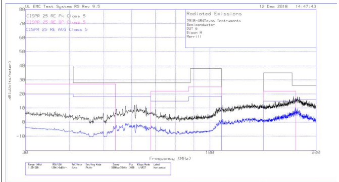
Figure 40. Radiated EMI Bicon Horizontal vs. CISPR25 Limits
