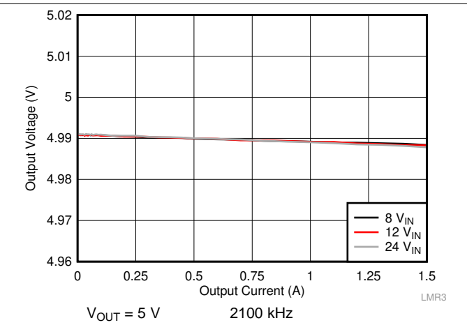
Figure 47. Load Regulation
