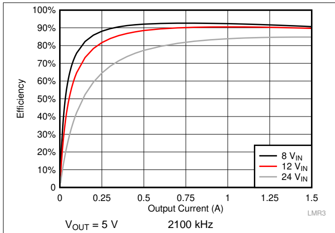
Figure 46. Efficiency
