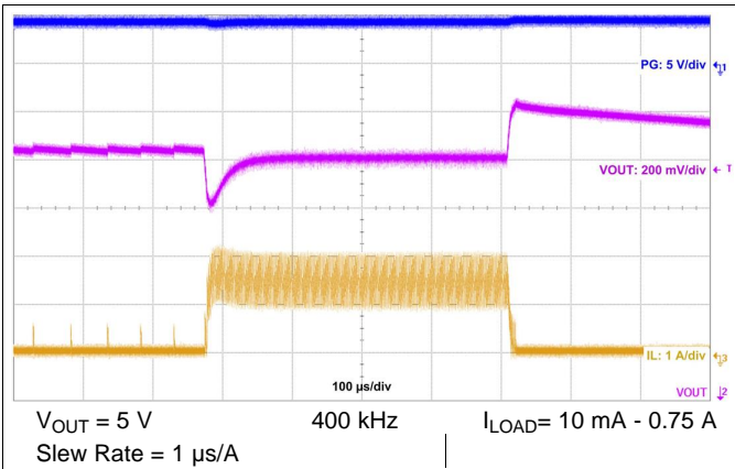
Figure 34. Load Transient
