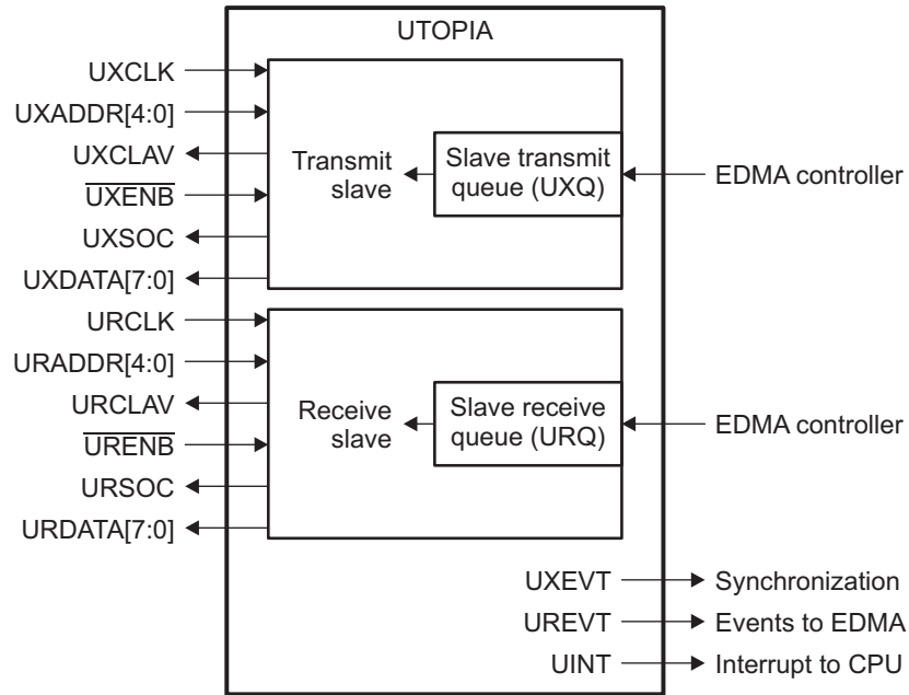
Figure 2. UTOPIA Block Diagram
