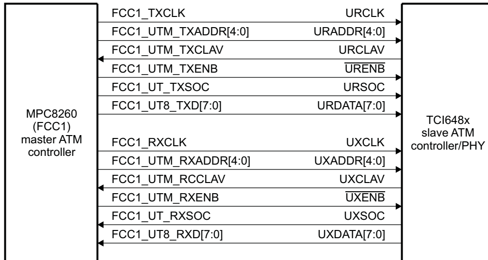
Figure 4. UTOPIA Slave Interfaced to Motorola MPC8260 Power QUICC IIE™ Master in 8-Bit Mode
