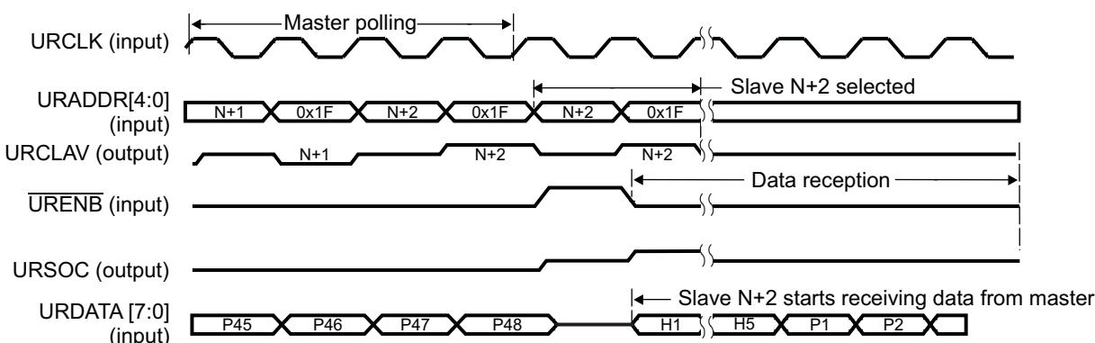
Figure 6. ATM Controller Slave Receive Timing Diagram
