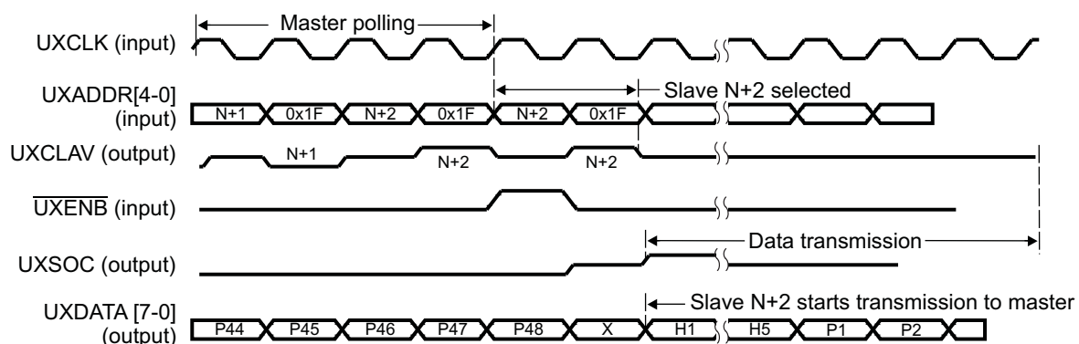
Figure 5. ATM Controller Slave Transmit Timing Diagram
