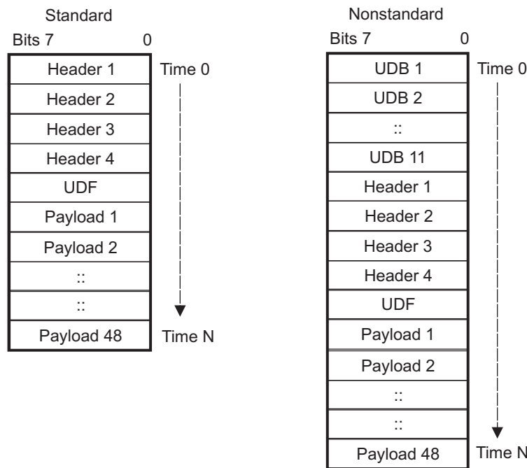
Figure 3. Cell Transfer Formats for 8-Bit Mode
