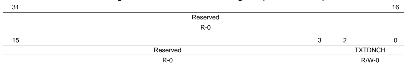
Figure 43. Transmit Teardown Register (TXTEARDOWN)
