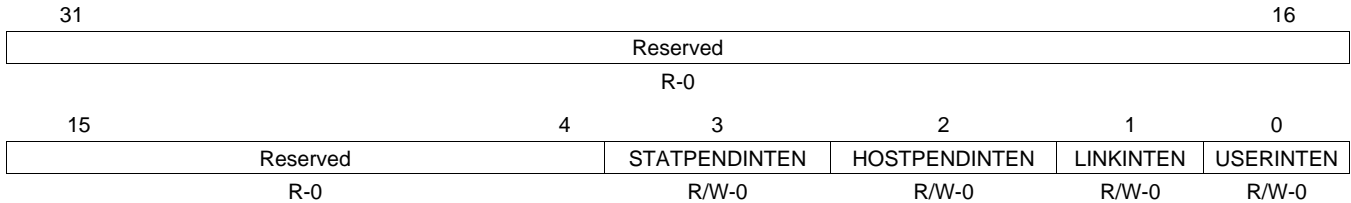
Figure 20. EMAC Control Module Miscellaneous Interrupt Enable Register (CMMISCINTEN)
