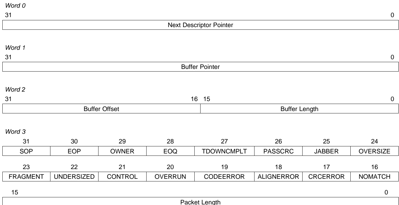
Figure 8. Receive Buffer Descriptor Format
