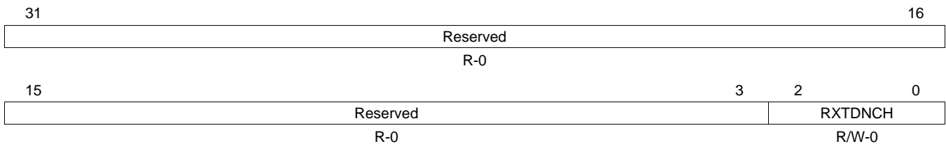
Figure 46. Receive Teardown Register (RXTEARDOWN)
