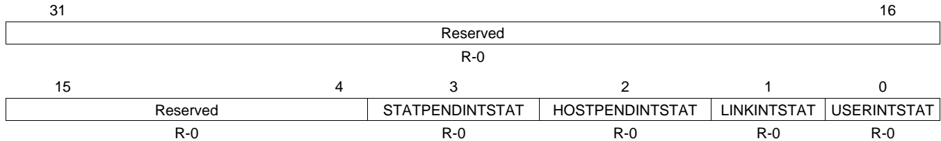
Figure 24. EMAC Control Module Miscellaneous Interrupt Status Register (CMMISCINTSTAT)
