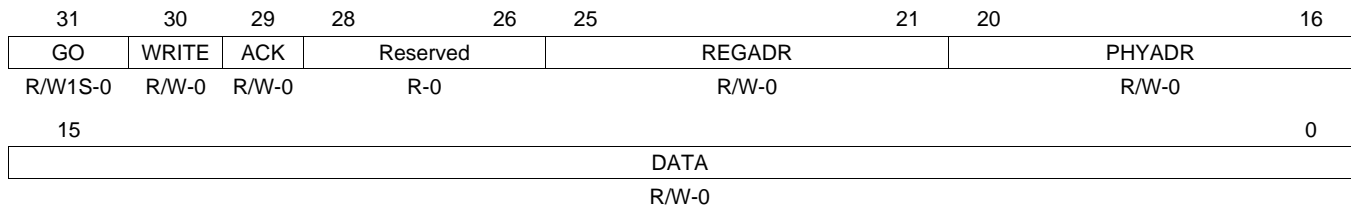
Figure 39. MDIO User Access Register 1 (USERACCESS1)
