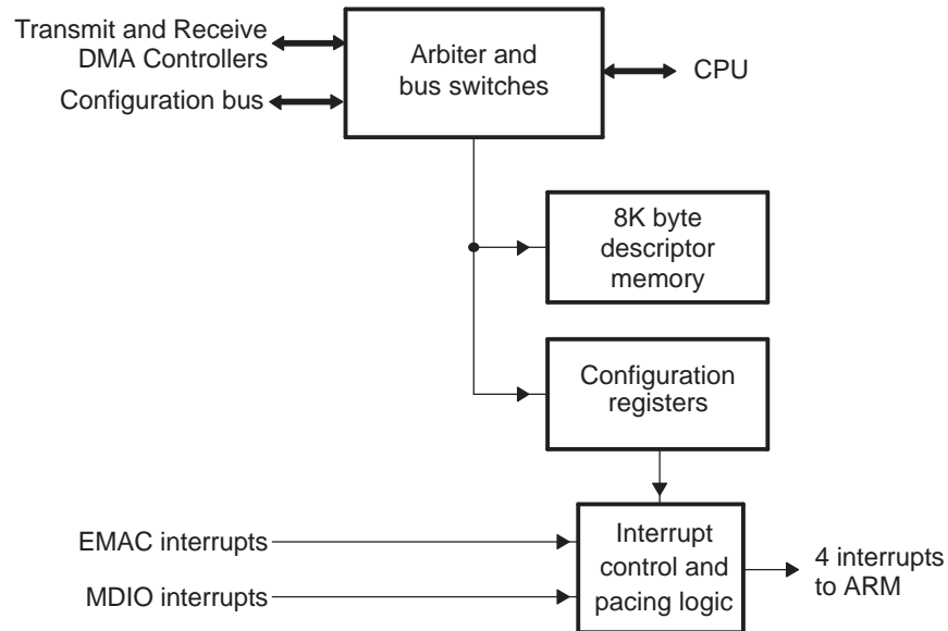
Figure 9. EMAC Control Module Block Diagram
