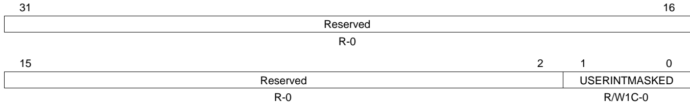
Figure 34. MDIO User Command Complete Interrupt (Masked) Register (USERINTMASKED)
