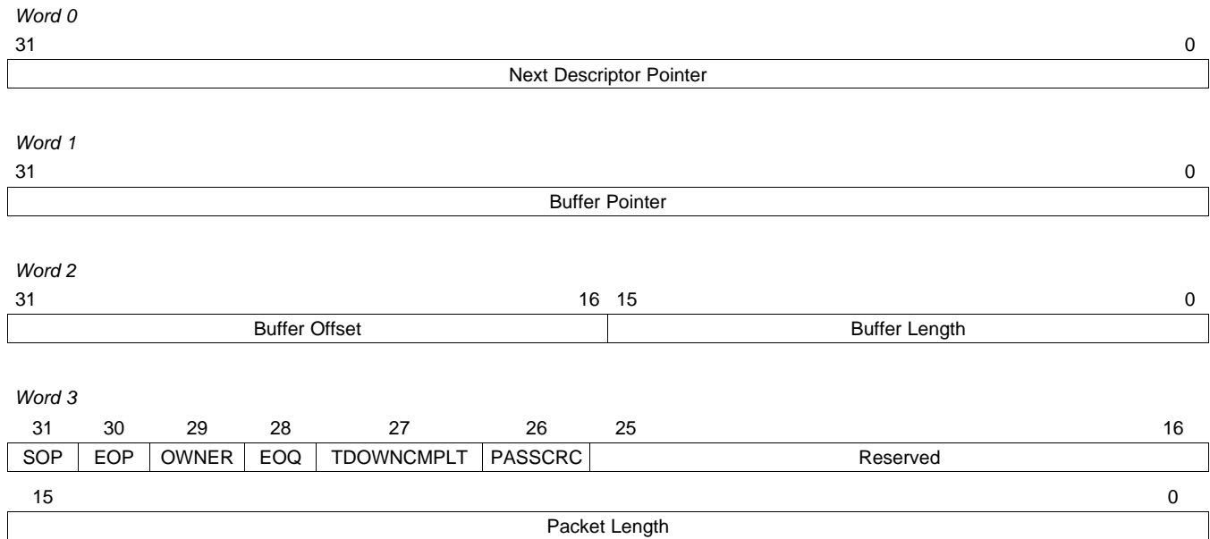
Figure 7. Transmit Buffer Descriptor Format
