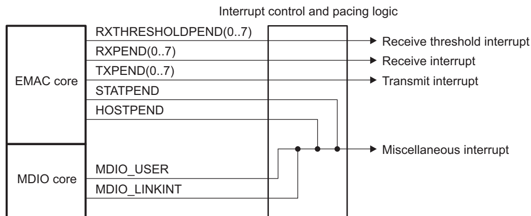
Figure 12. EMAC Control Module Interrupt Logic Diagram
