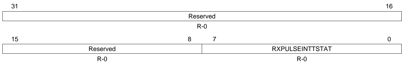
Figure 22. EMAC Control Module Receive Interrupt Status Register (CMRXINTSTAT)
