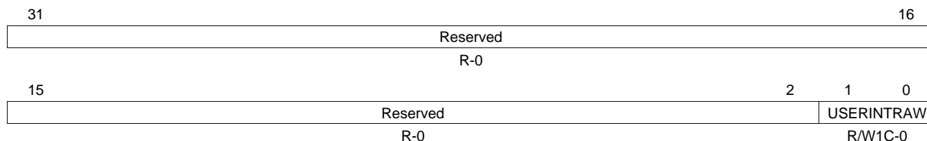
Figure 33. MDIO User Command Complete Interrupt (Unmasked) Register (USERINTRAW)
