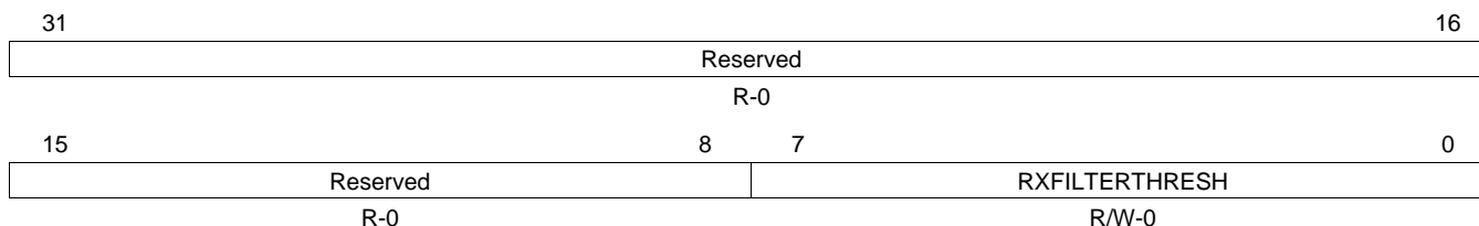
Figure 66. Receive Filter Low Priority Frame Threshold Register (RXFILTERLOWTHRESH)
