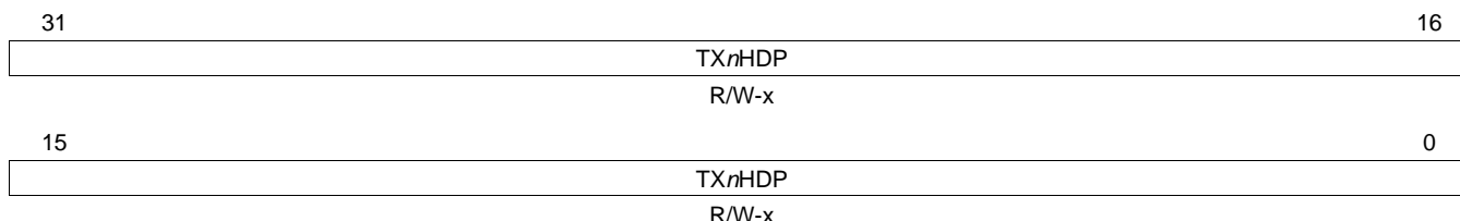
Figure 86. Transmit Channel n DMA Head Descriptor Pointer Register (TXnHDP)
