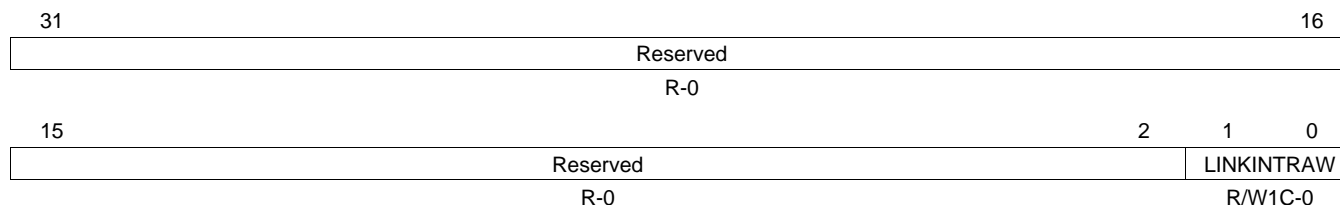
Figure 31. MDIO Link Status Change Interrupt (Unmasked) Register (LINKINTRAW)
