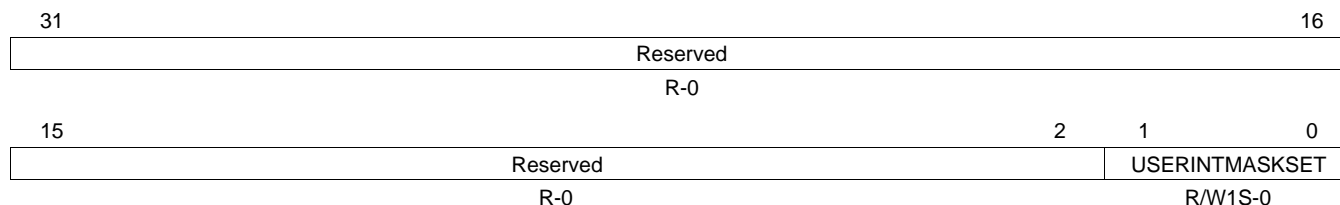
Figure 35. MDIO User Command Complete Interrupt Mask Set Register (USERINTMASKSET)
