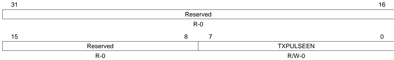
Figure 19. EMAC Control Module Transmit Interrupt Enable Register (CMTXINTEN)
