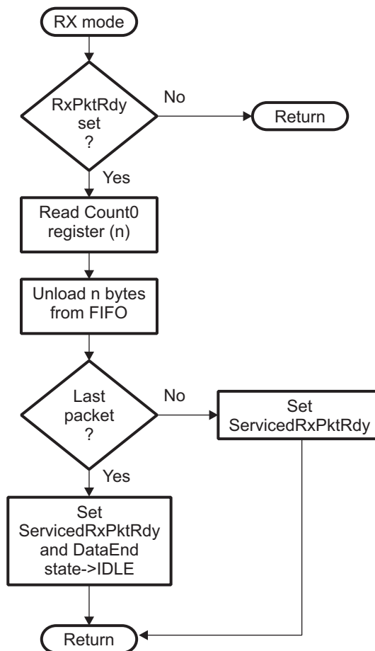
Figure 10. RX Mode Flow Chart
